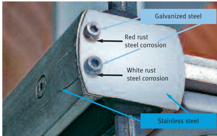
Figure 15: Fastening of a stainless steel cover (on a facade assembly) using galvani- zed screws: the screws show white rust and in- itial discolouration (steel corrosion) after one year in urban atmosphere
