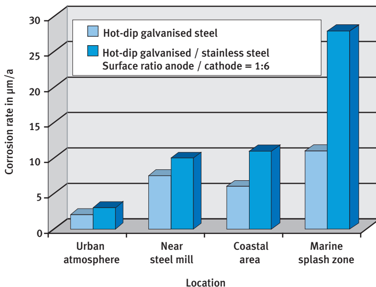
Figure 6: Corrosion rates of hot-dip galvanized steel, with and without contact with stainless steel, in different environments
